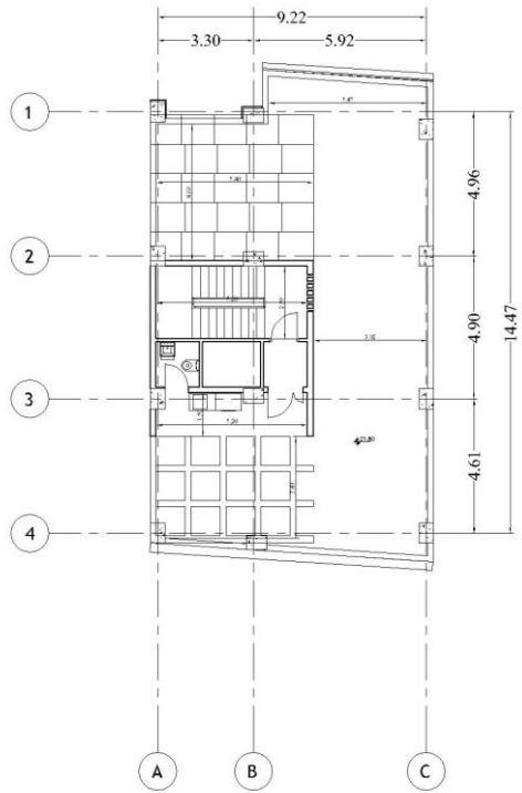
DIMENTION PLAN - ROOF GARDEN
