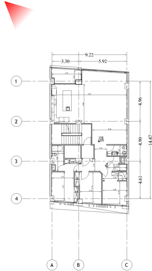
DIMENTION PLAN - L1,2,4,5
