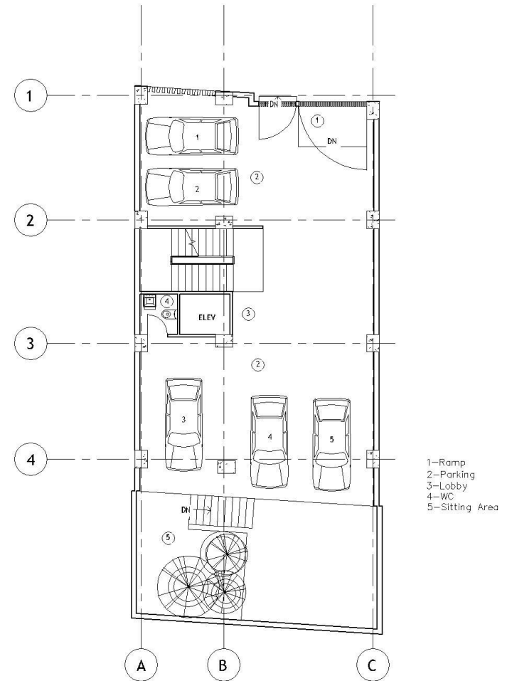
FURNITURE PLAN - GF
