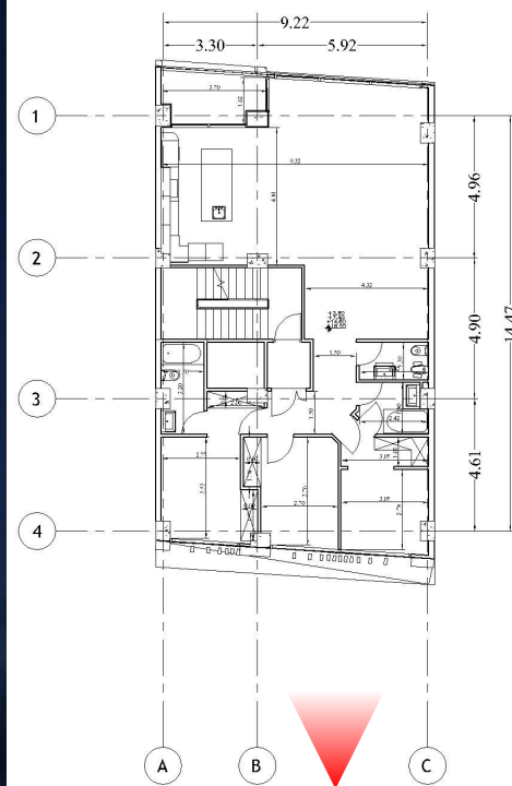
DIMENTION PLAN - L1,2,4,5
