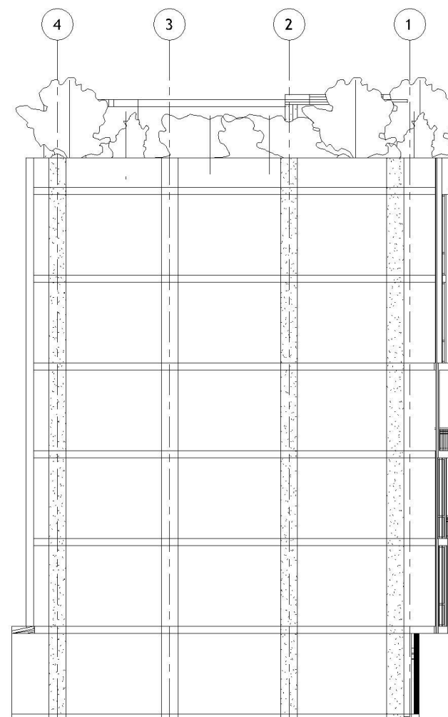
EAST ELEVATION
