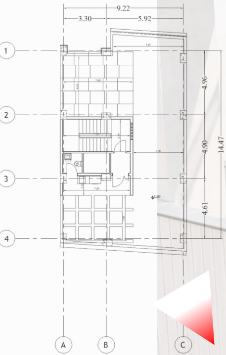
DIMENTION PLAN - ROOF GARDEN
