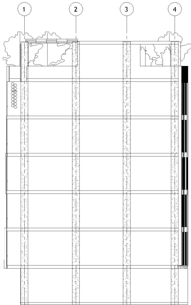
WEST ELEVATION
