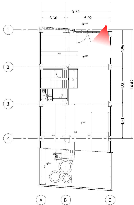
DIMENTION PLAN - GF
