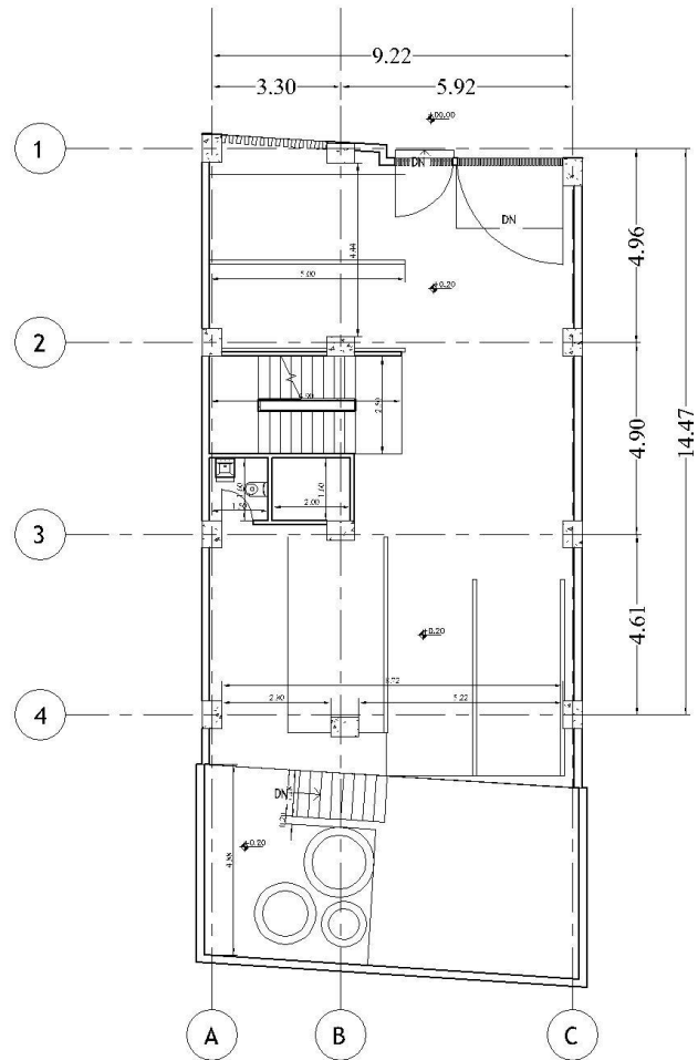
DIMENTION PLAN - GF
