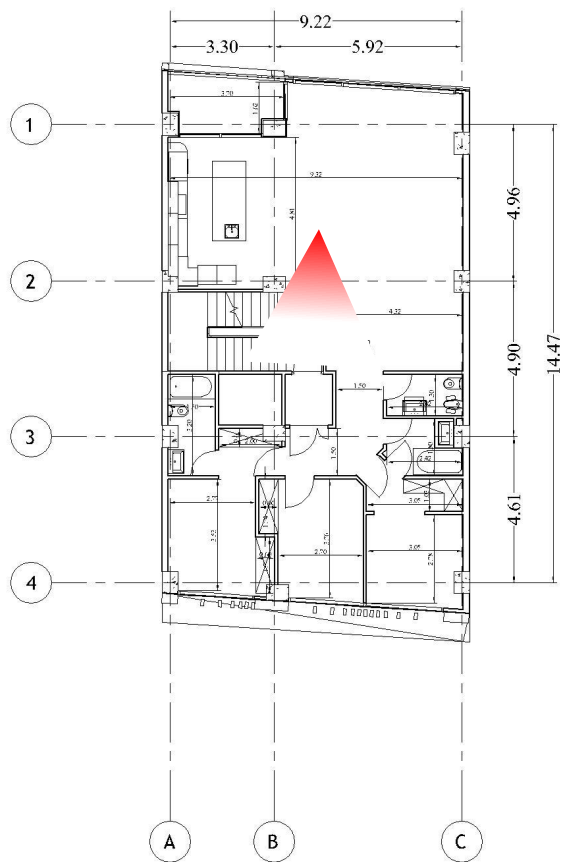
DIMENTION PLAN - L1,2,4,5
