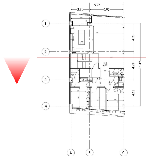
DIMENTION PLAN - L1,2,4,5
