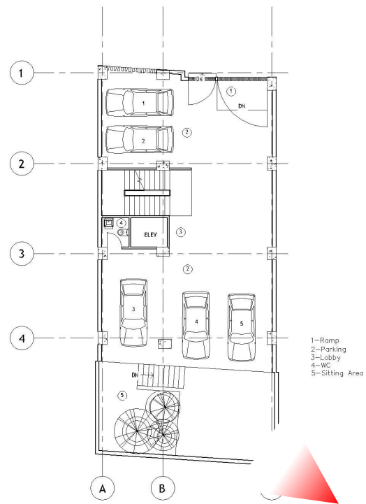
FURNITURE PLAN - GF
