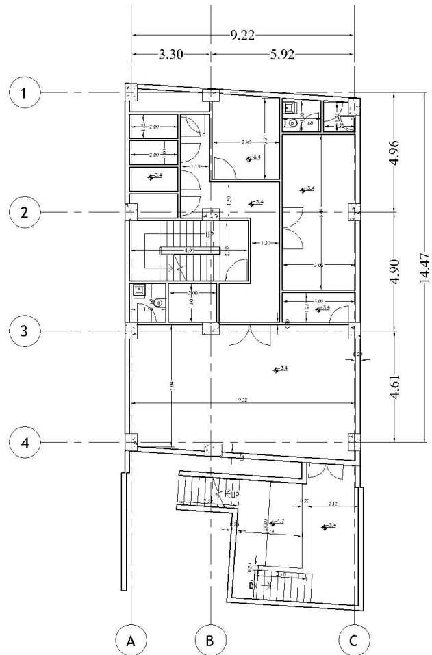
DIMENTION PLAN - BASEMENT
