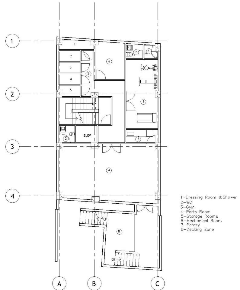
FURNITURE PLAN - BASEMENT
