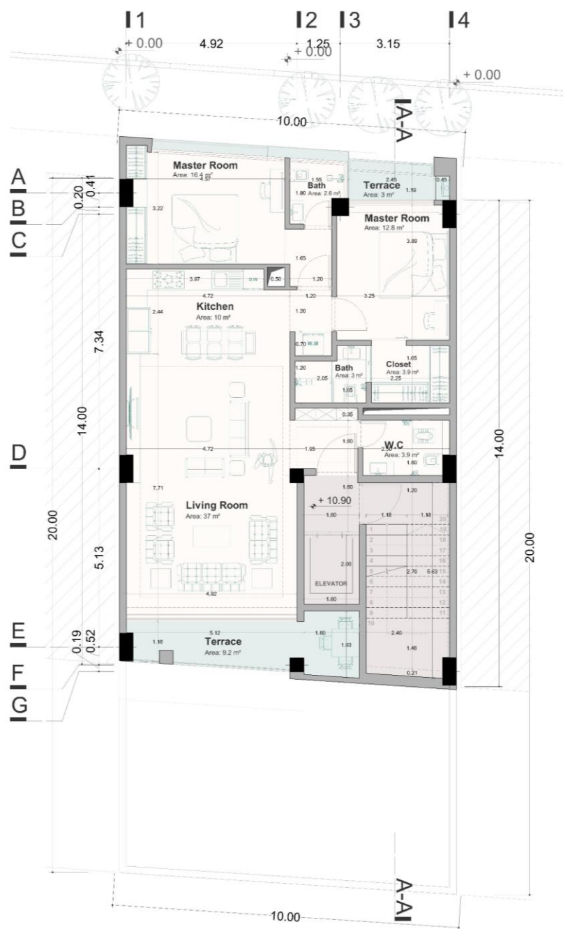
3th Floor Plan
