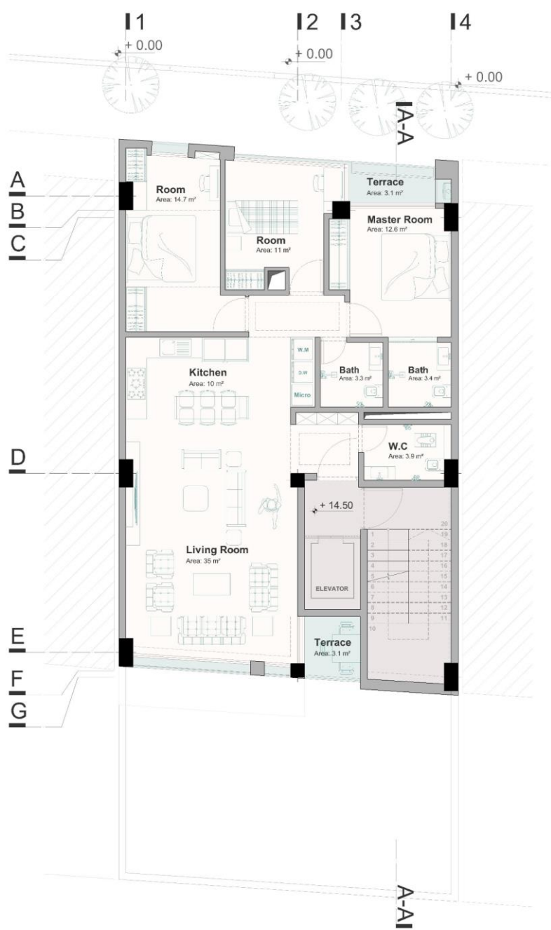
4th Floor Plan
