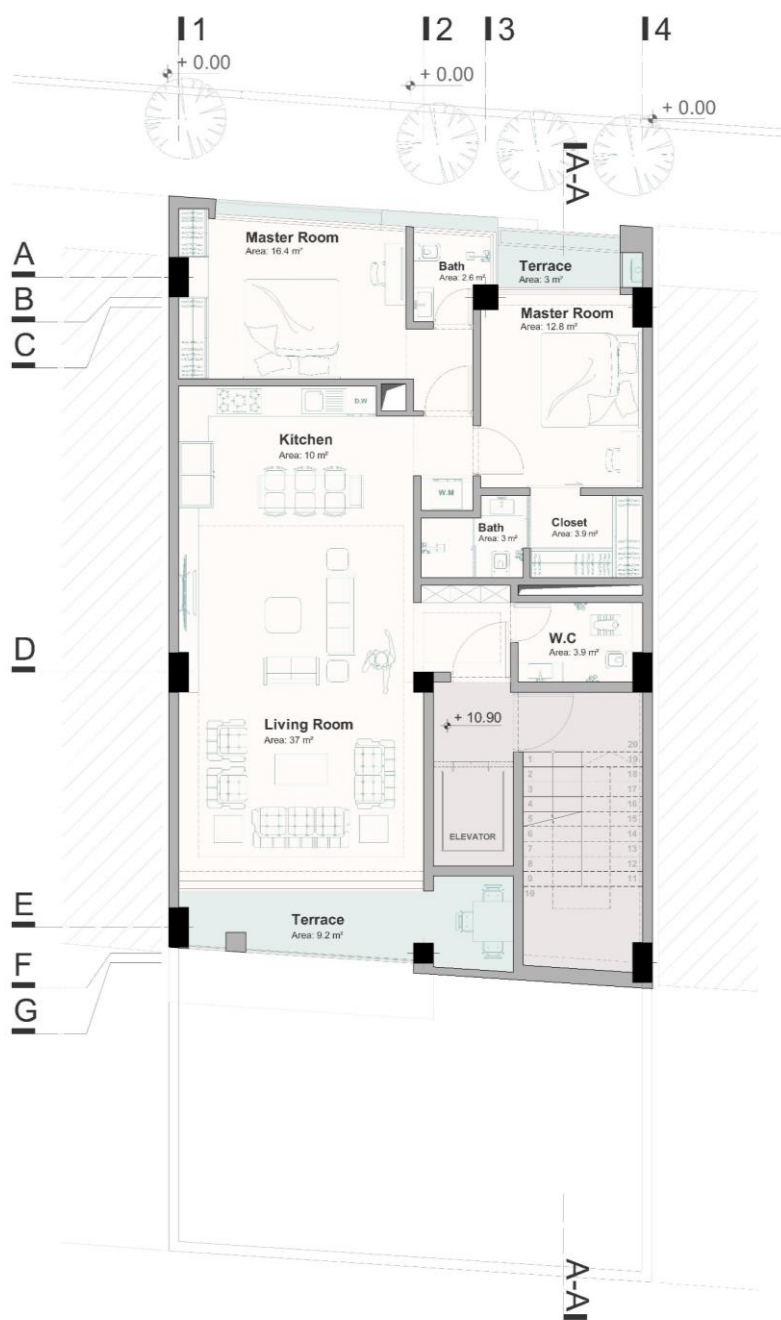
3th Floor Plan
