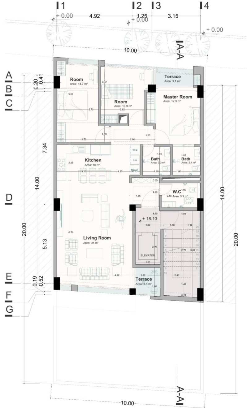
1th Floor Plan
