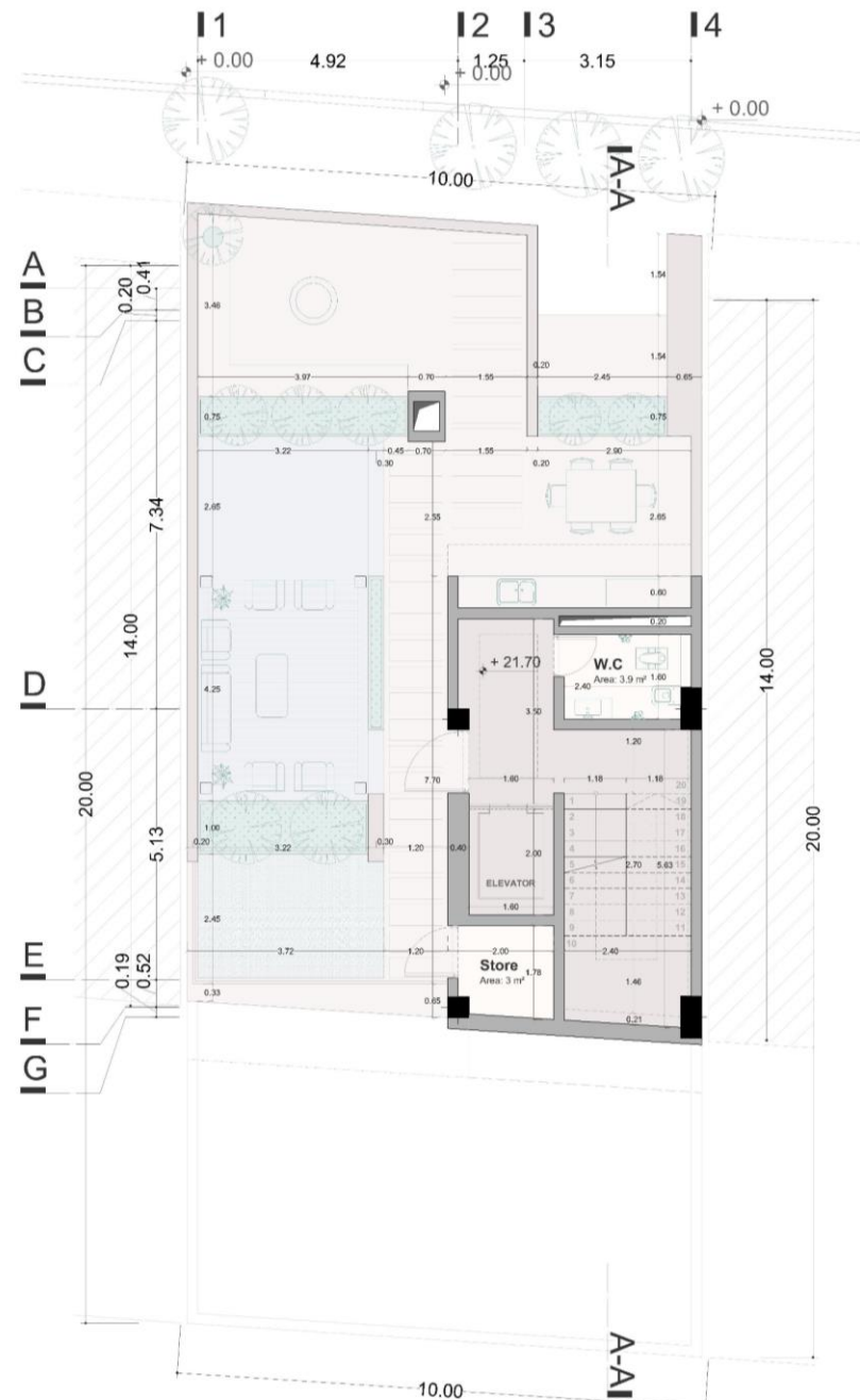
Roof Floor Plan
