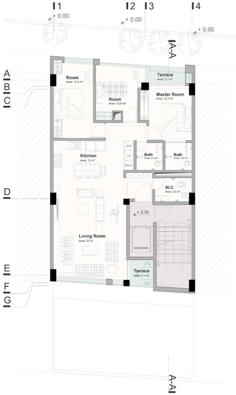
1th Floor Plan
