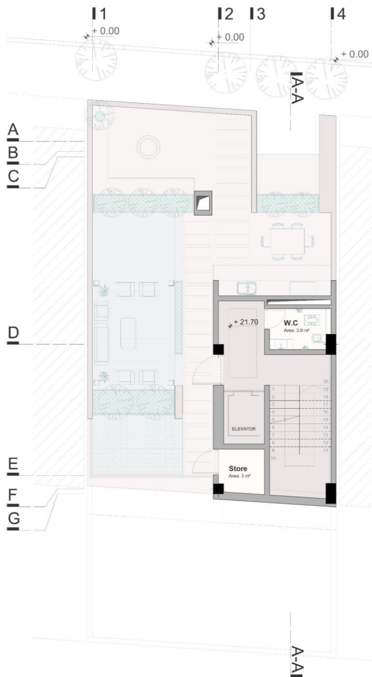
Roof Floor Plan
