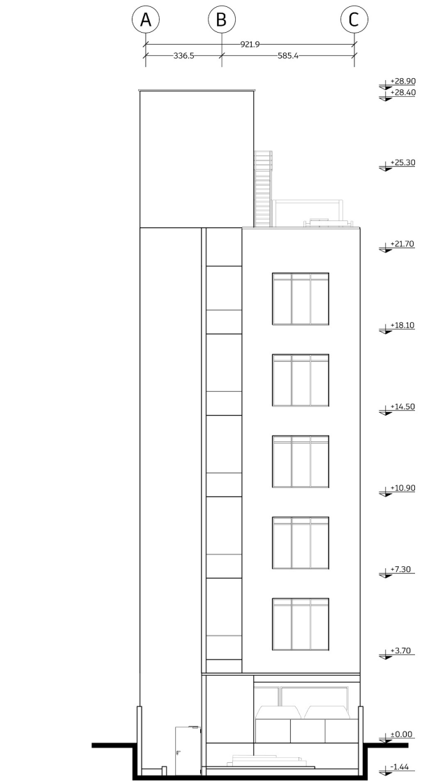
South Facade 0 1 2 3 4 5 10 m
