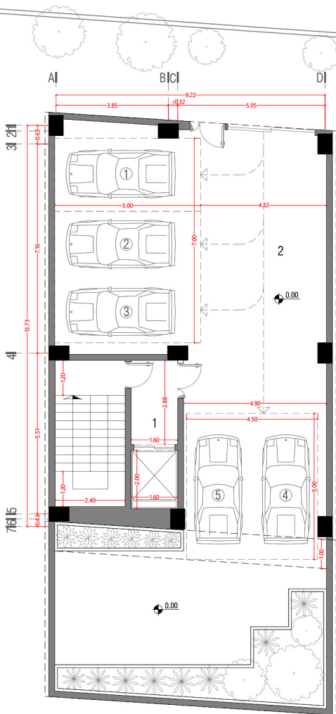
Ground Floor Dimension Plan
