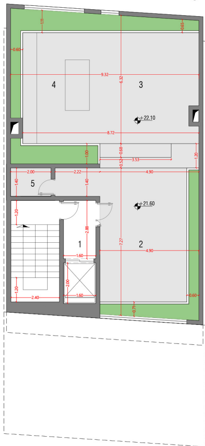
Roof Garden Dimension Plan
