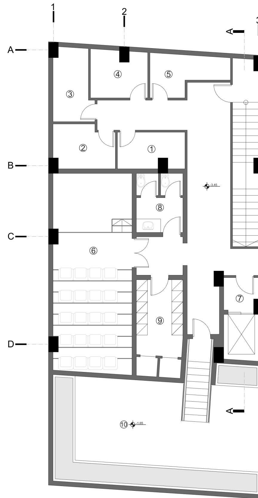
Under Ground Floor Plan
