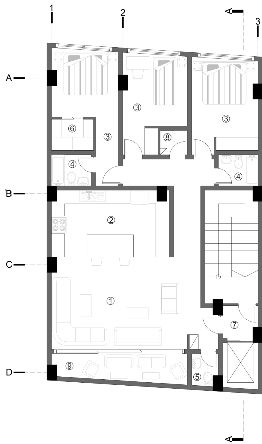
Three Bed Rooms Units Plan (Height Code : +7.35 , +10.95 , +14.55 , +18.15)
