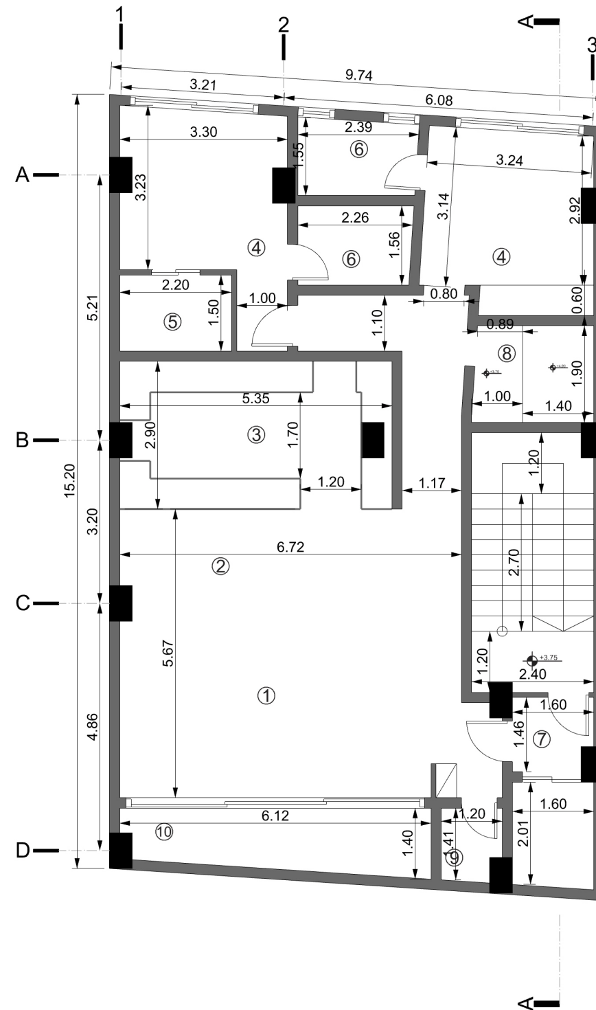
Two Bed Rooms Unit Plan
