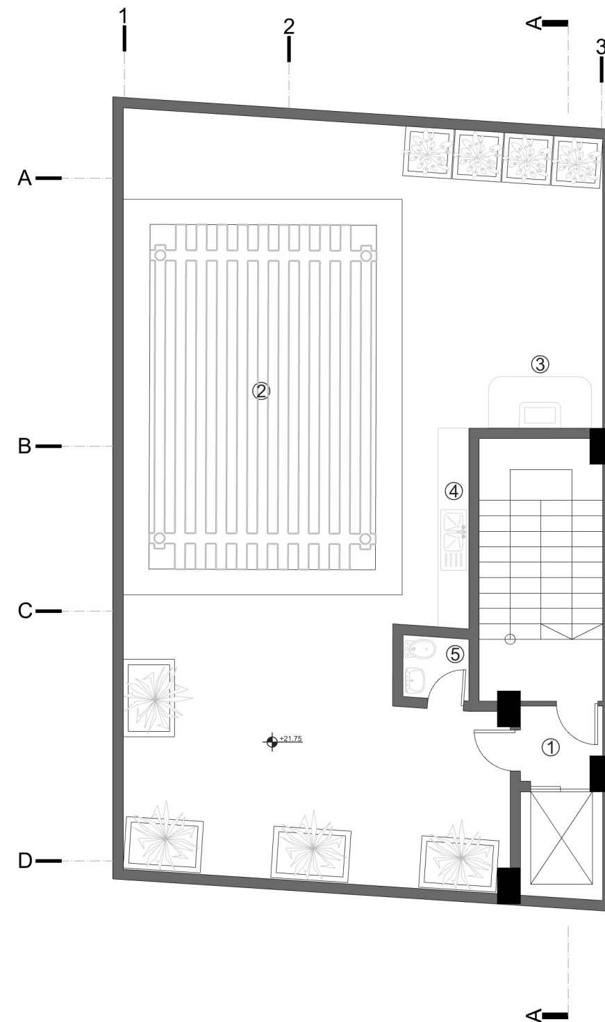
Roof Plan
