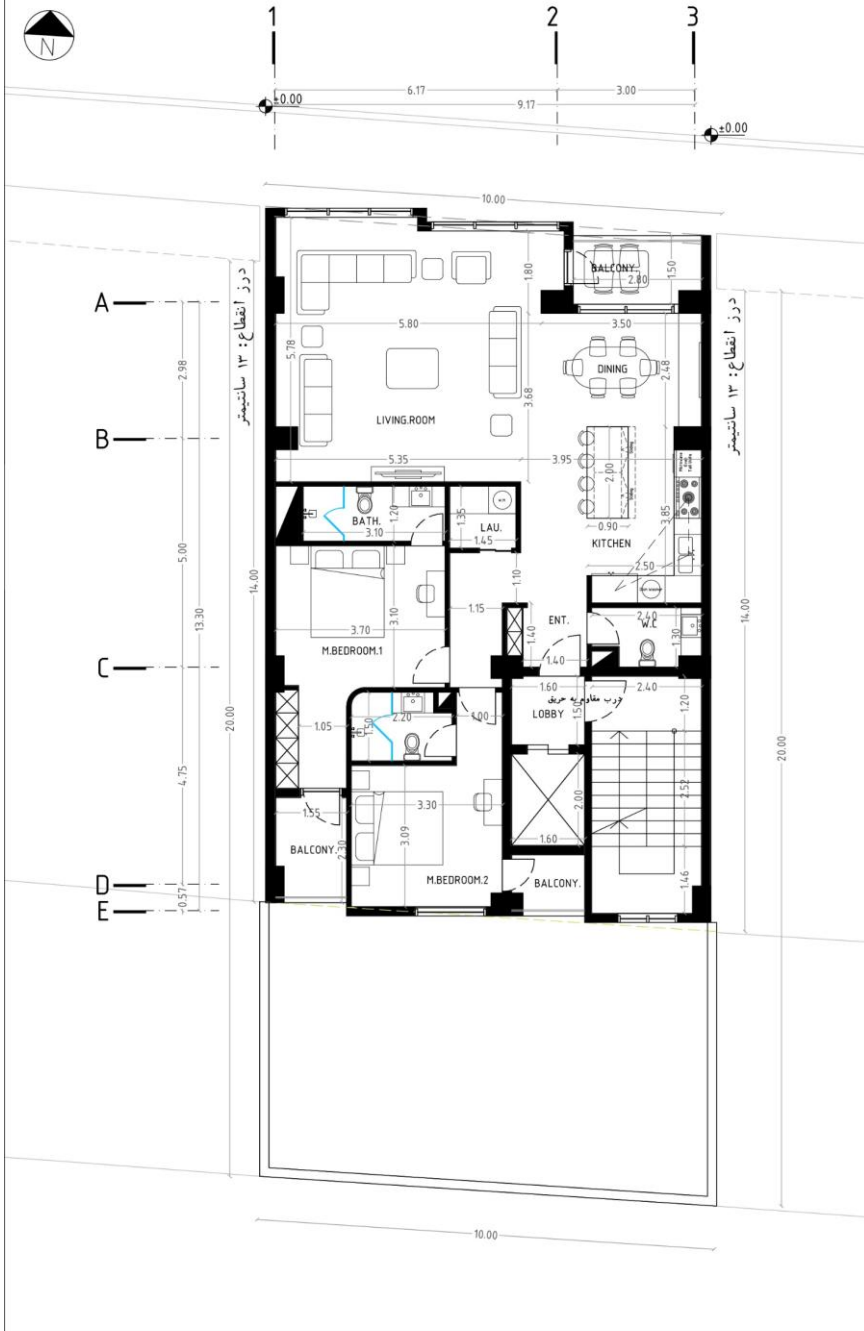
3RD FLOOR DIMENSION PLAN
