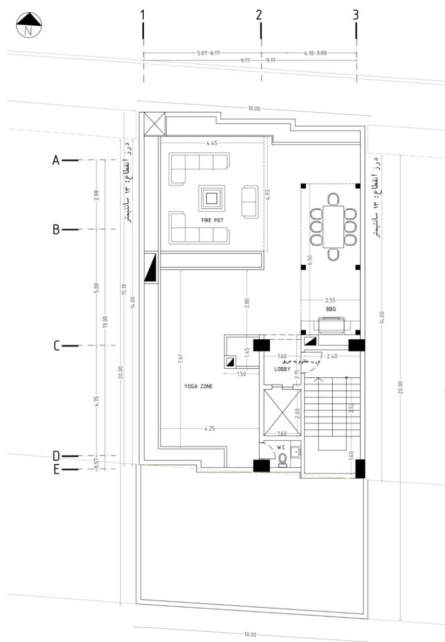
ROOF GARDEN FLOOR DIMENSION PLAN
