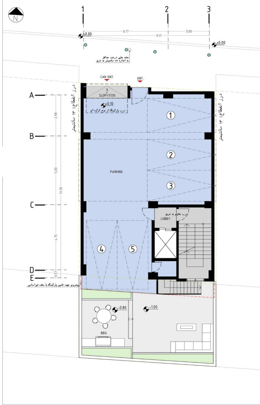
GROUND FLOOR FURNITURE PLAN
