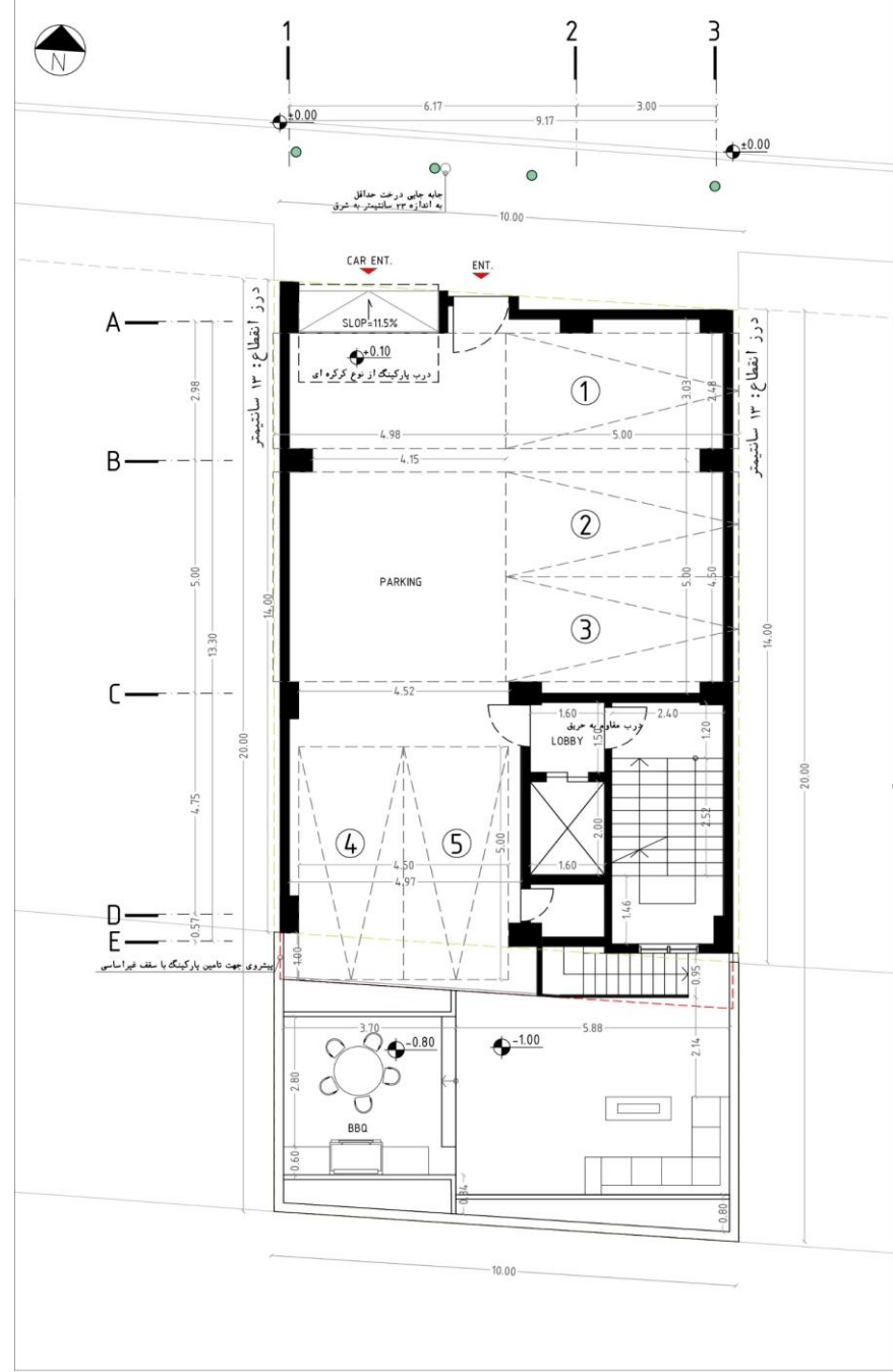
GROUND FLOOR DIMENSION PLAN
