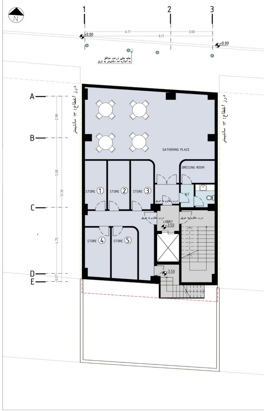
BASEMENT FLOOR FURNITURE PLAN
