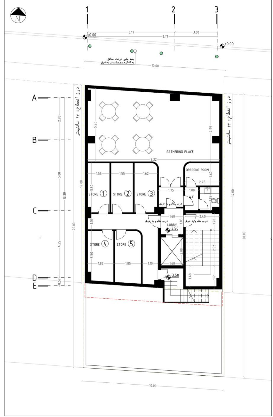
BASEMENT FLOOR DIMENSION PLAN
