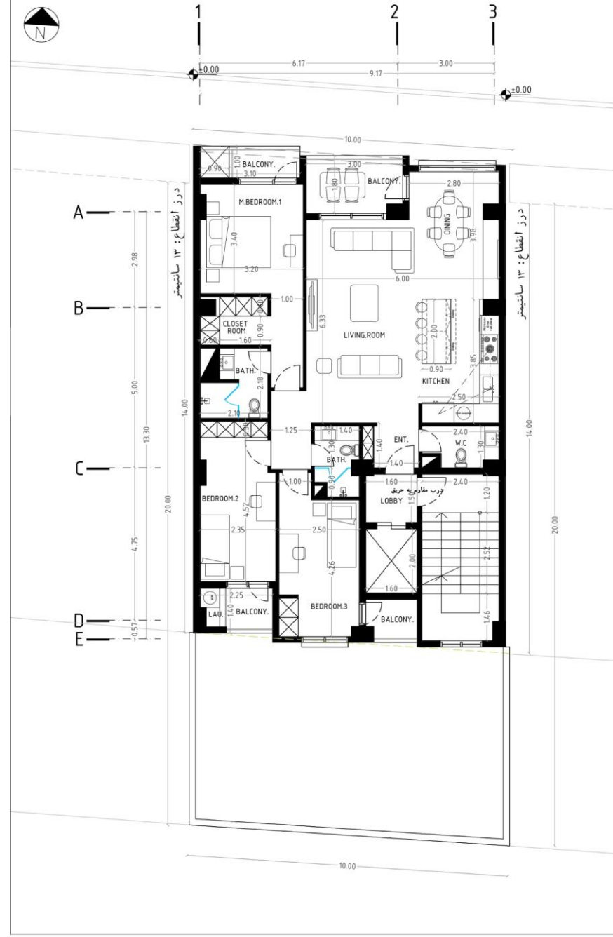
2ND FLOOR DIMENSION PLAN
