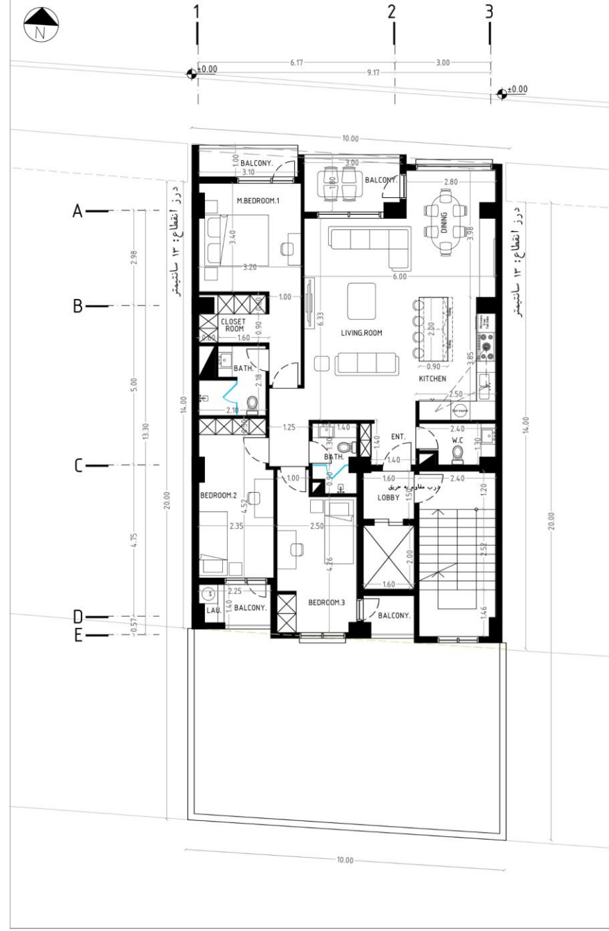
1ST 4TH 5TH FLOOR DIMENSION PLAN
