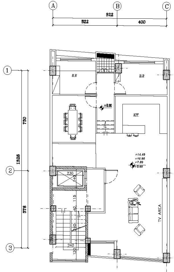
First Floor 2 B.R. sc: 1:100
