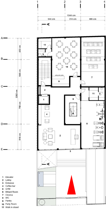
NIKSA RESIDENCE-ALT01
