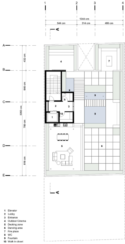
NIKSA RESIDENCE-ALT01
