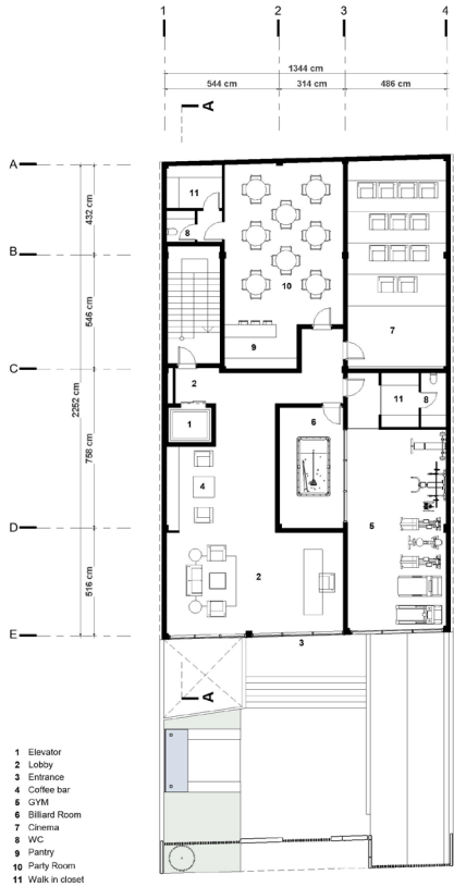
NIKSA RESIDENCE-ALT01
