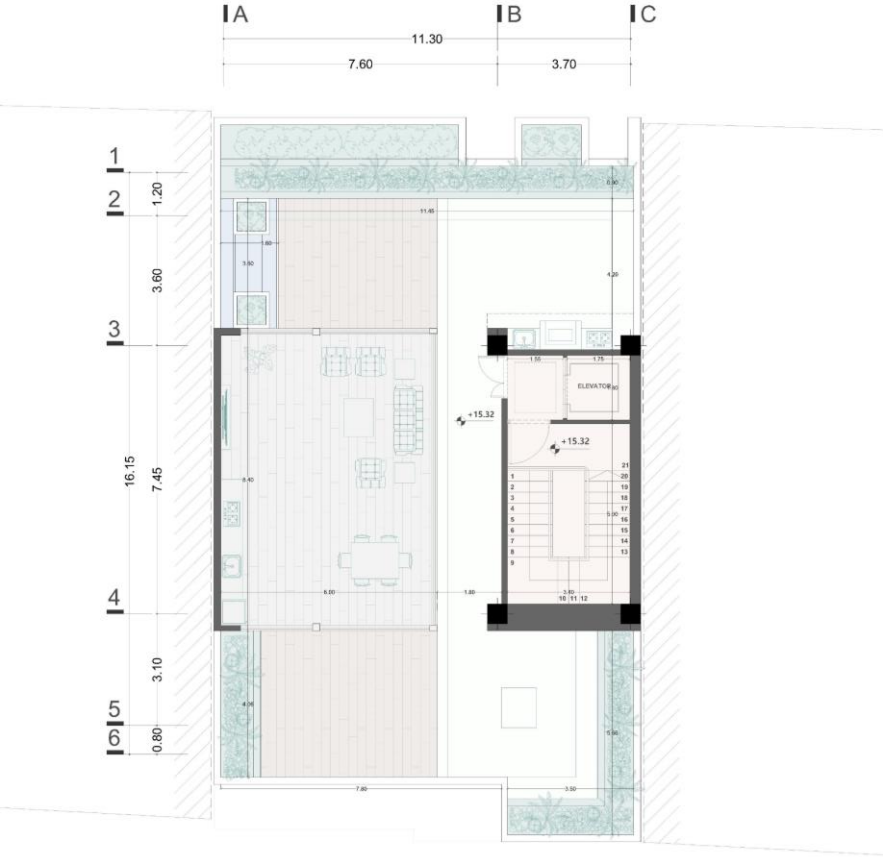
ROOF PLAN TOTAL AREA: 223 m²
