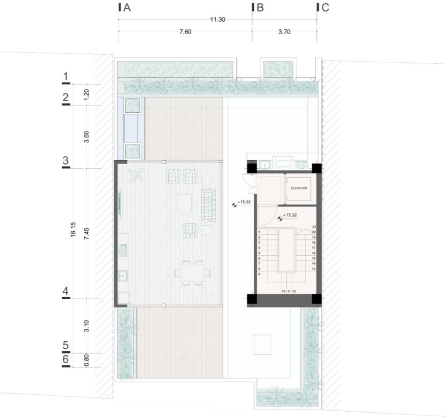
ROOF PLAN TOTAL AREA: 223 m²
