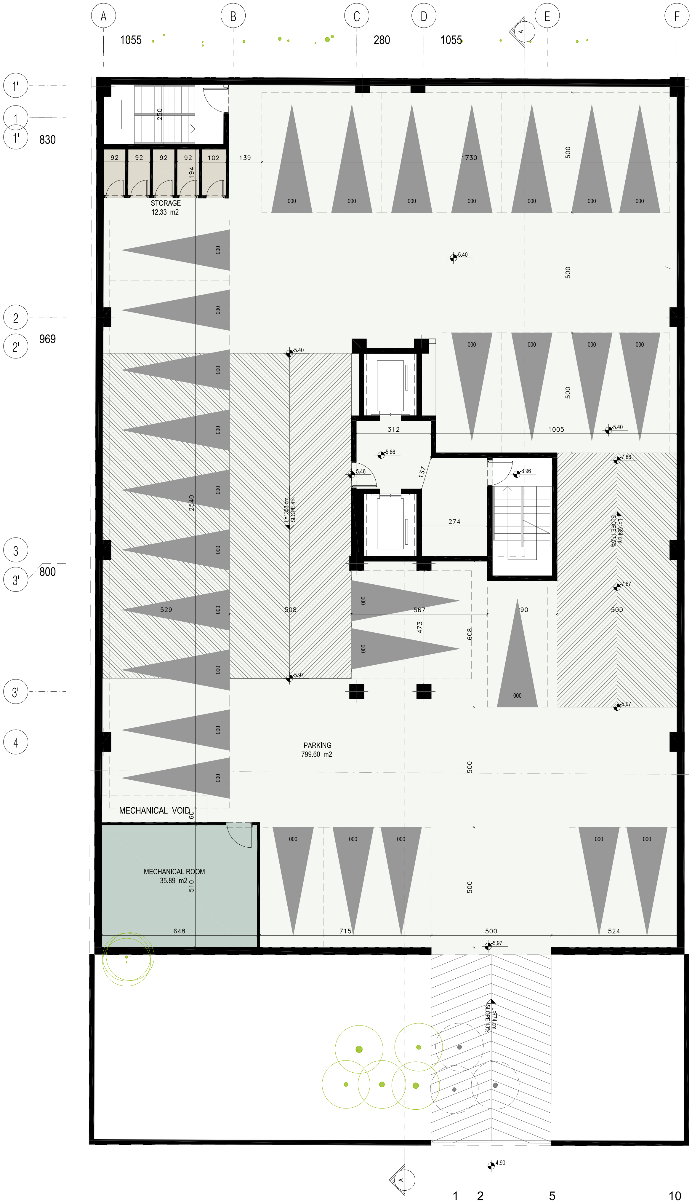
BASEMENT -2 TOTAL AREA | 775 M2 PARKING NUMBER | 29 ALL:81
