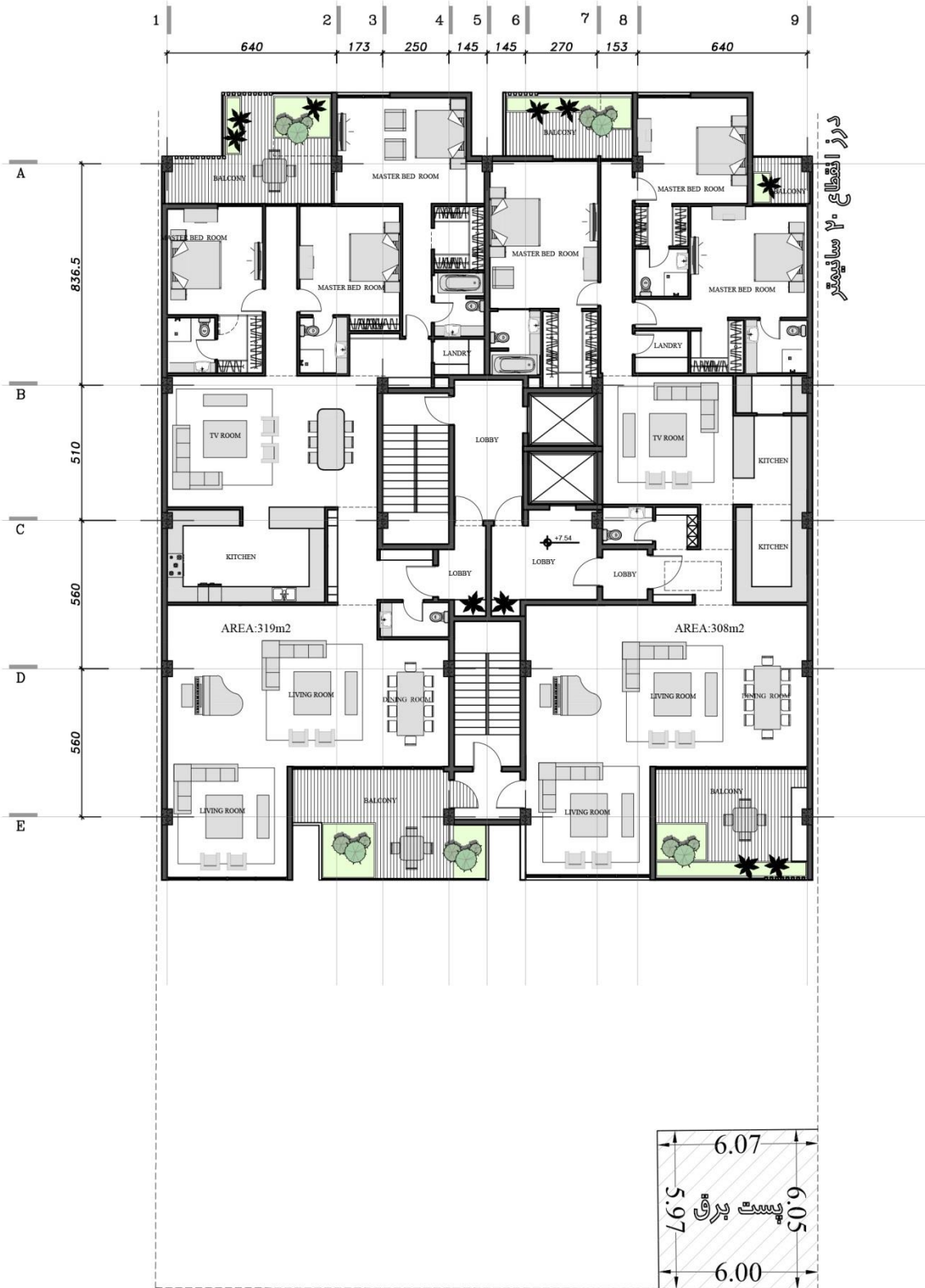
TYPICAL FLOOR PLAN ALT. 1
