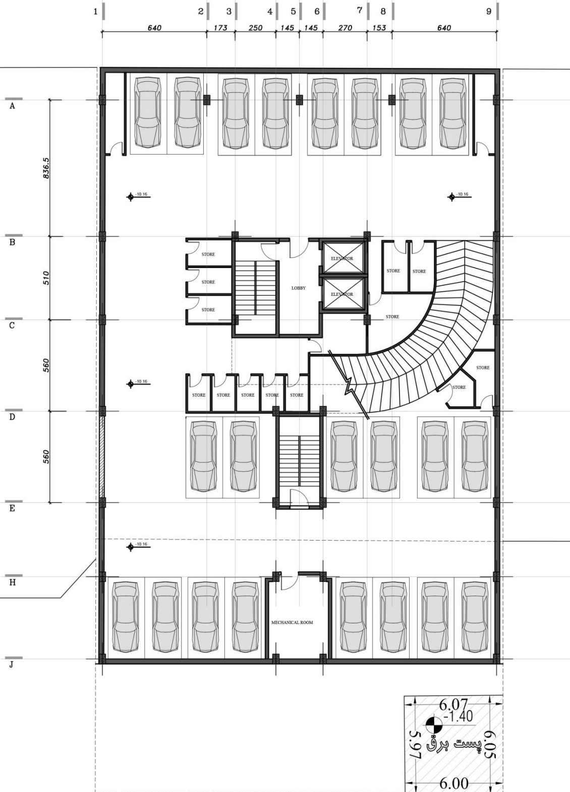
-3 FLOOR PLAN
