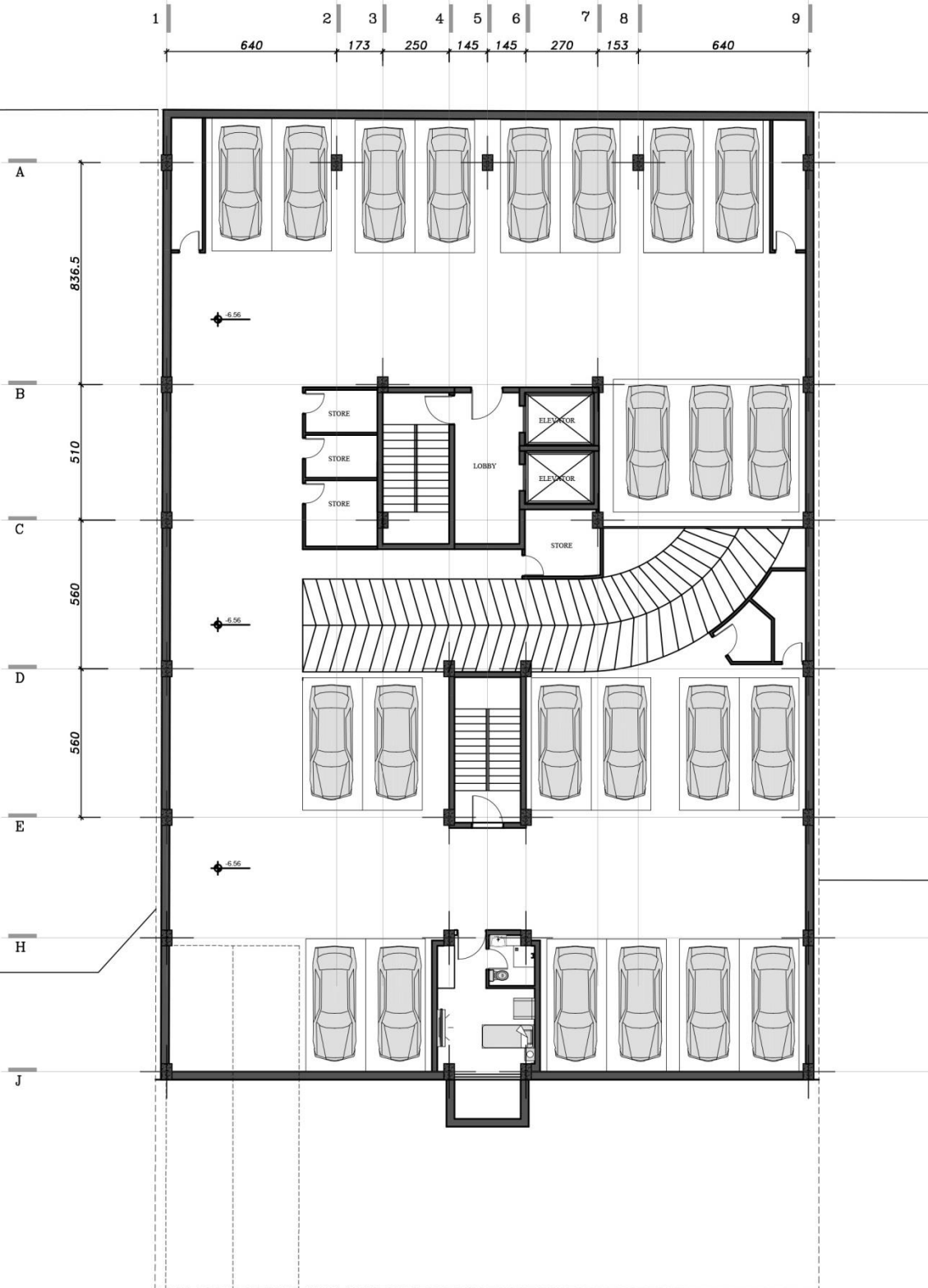
-2 FLOOR PLAN
