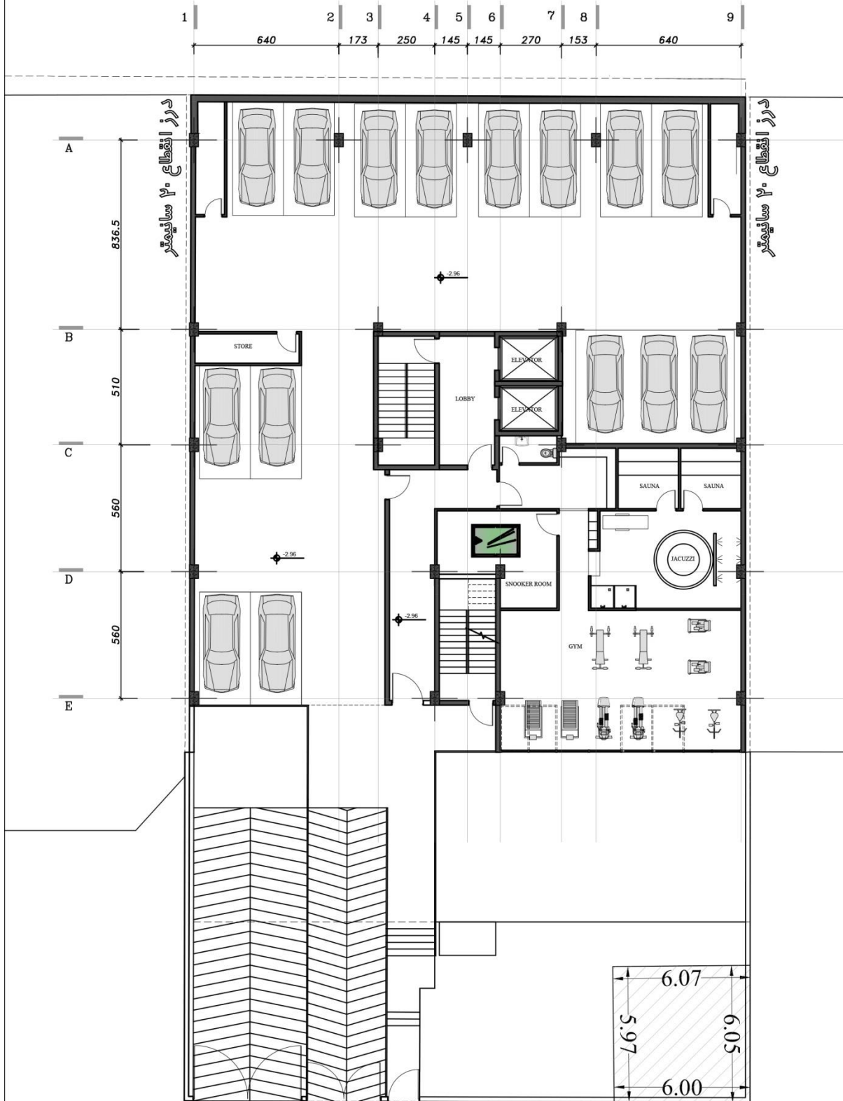
-1 FLOOR PLAN
