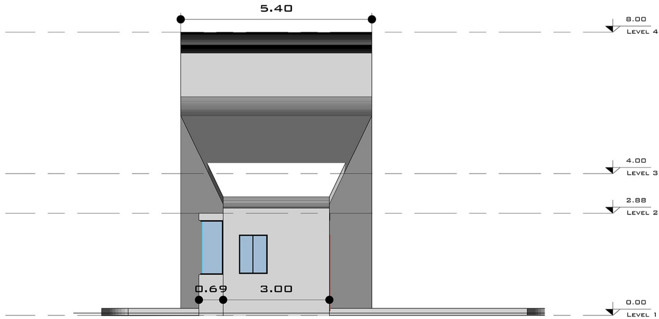
SECTION B-B
