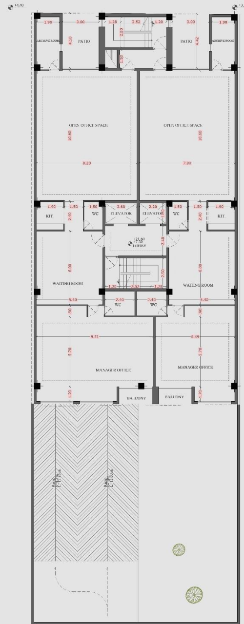
1ST & 5TH DIMENTION PLAN
