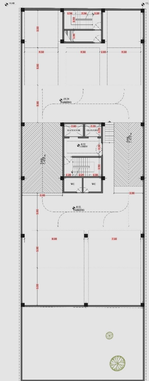
BASEMENT PLAN -3
