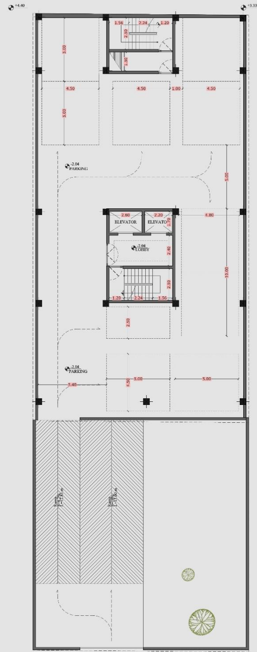
BASEMENT PLAN -1
