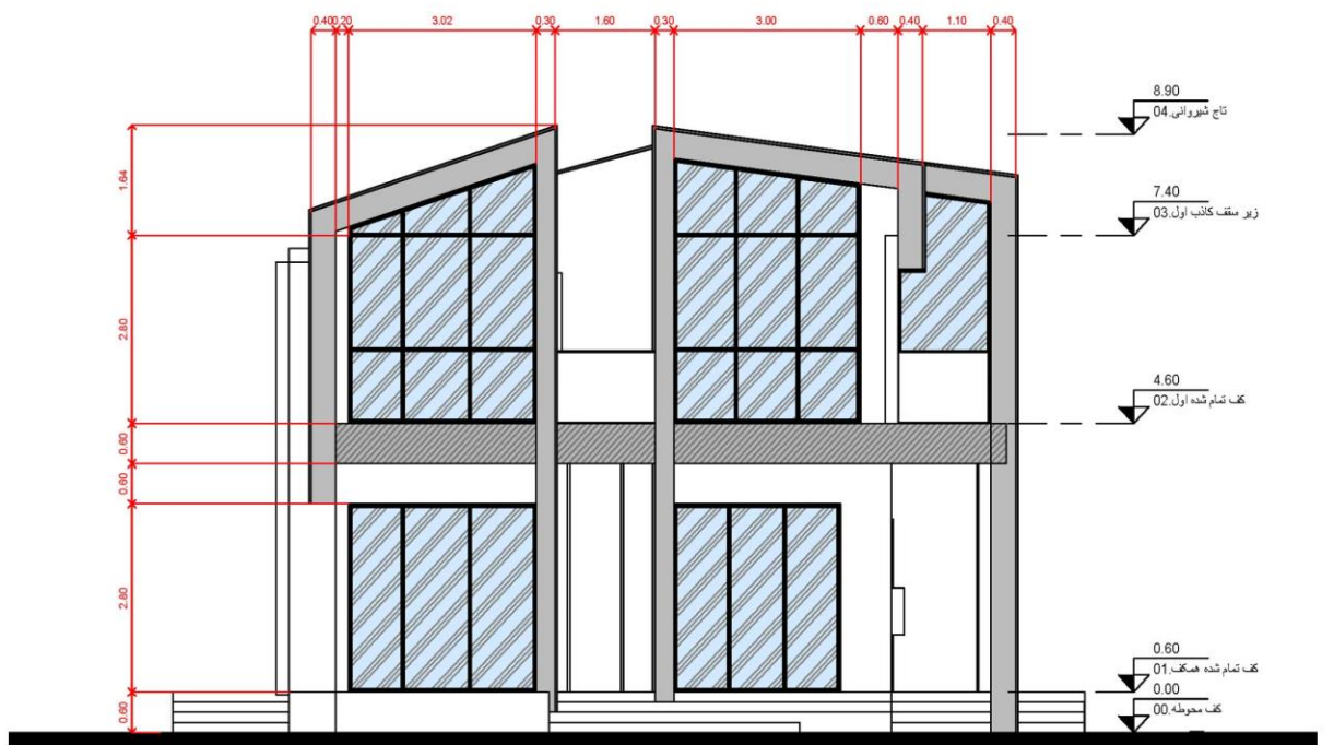
East elevation
