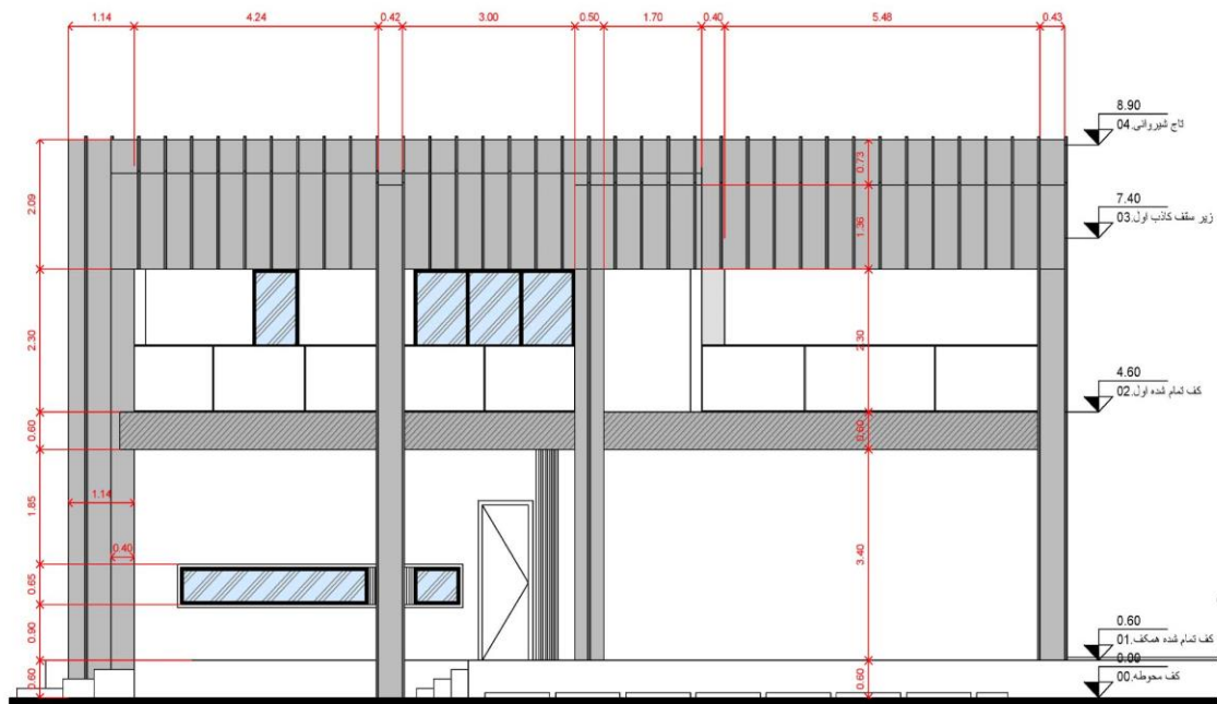
North elevation
