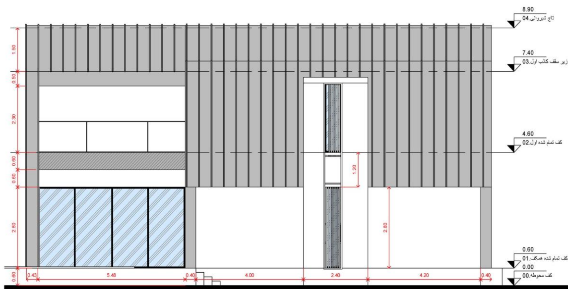
South elevation
