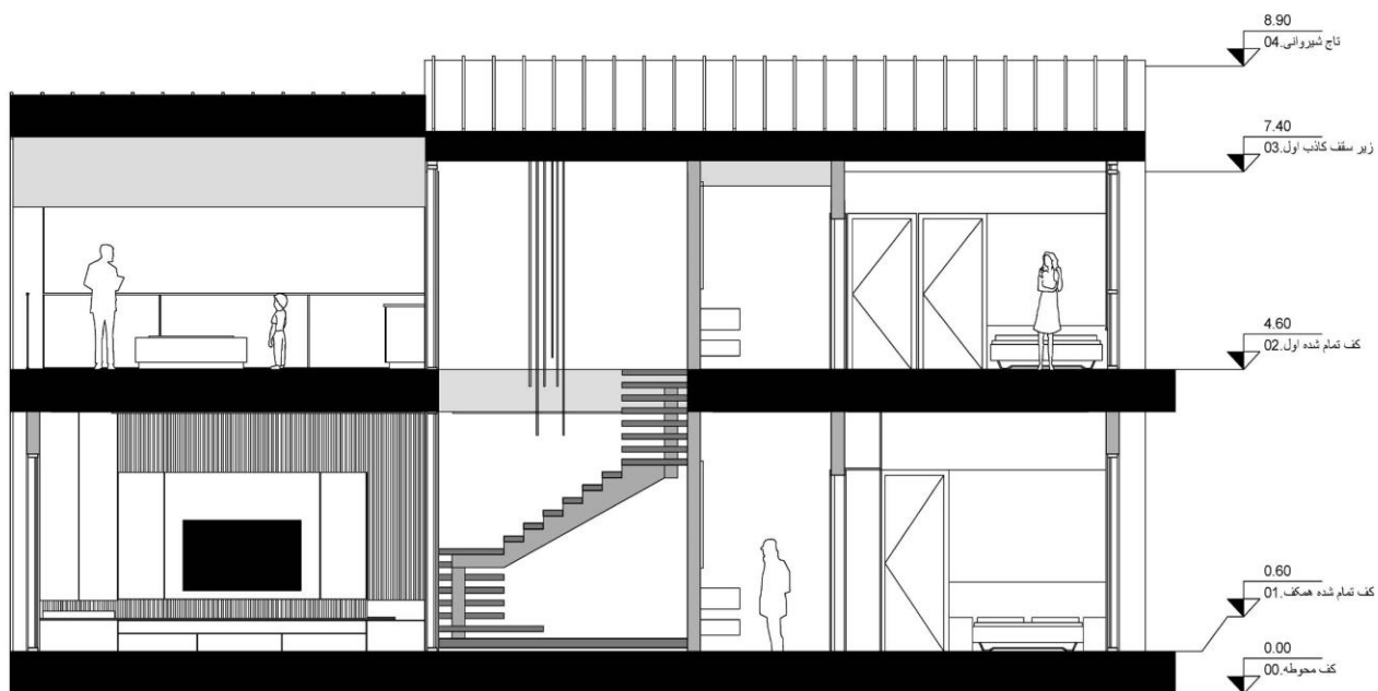
Section Line
