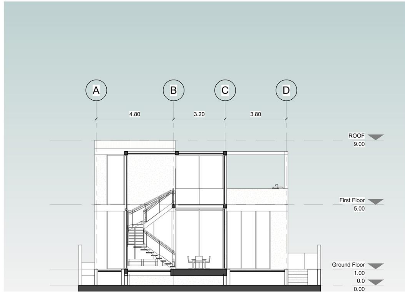
SECTION B-B
