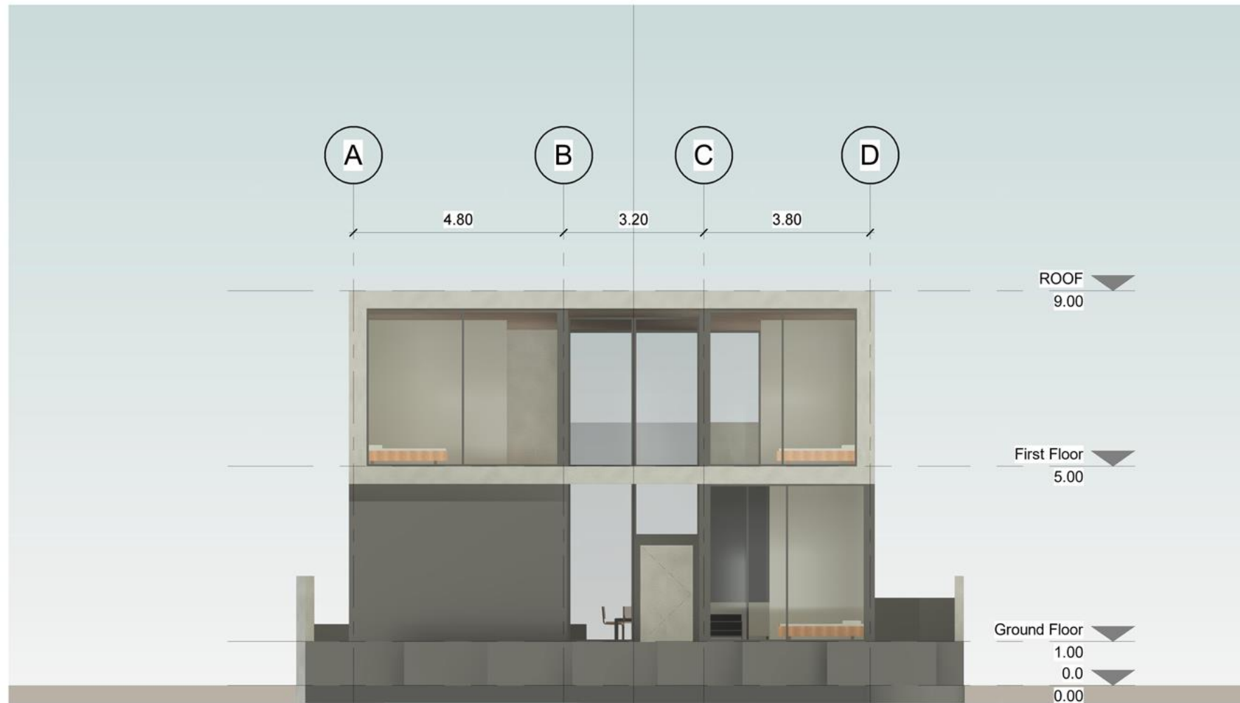
SOUTH ELEVATION
