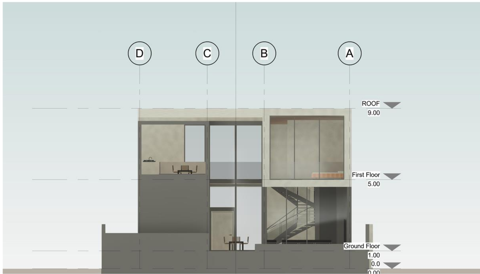
NORTH ELEVATION
