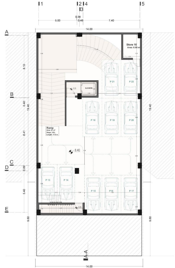
BASEMENT -3 TOTAL AREA: 324.69 m 2 NUMBER OF PARKING: 10
