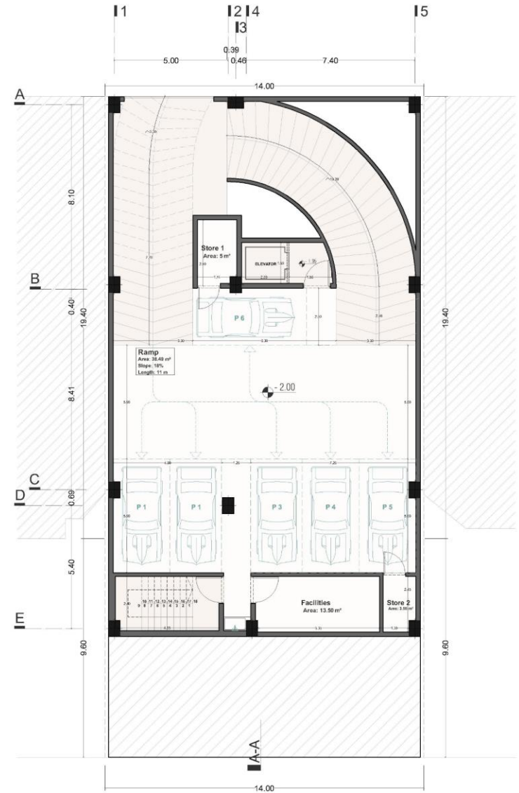
BASEMENT -1 TOTAL AREA: 324.69 m 2 NUMBER OF PARKING: 6
