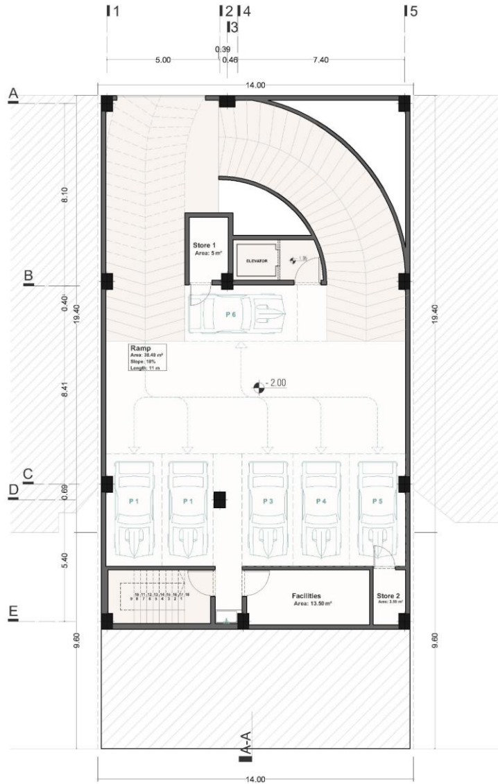
BASEMENT -1 TOTAL AREA: 324.69 m 2 NUMBER OF PARKING: 6
