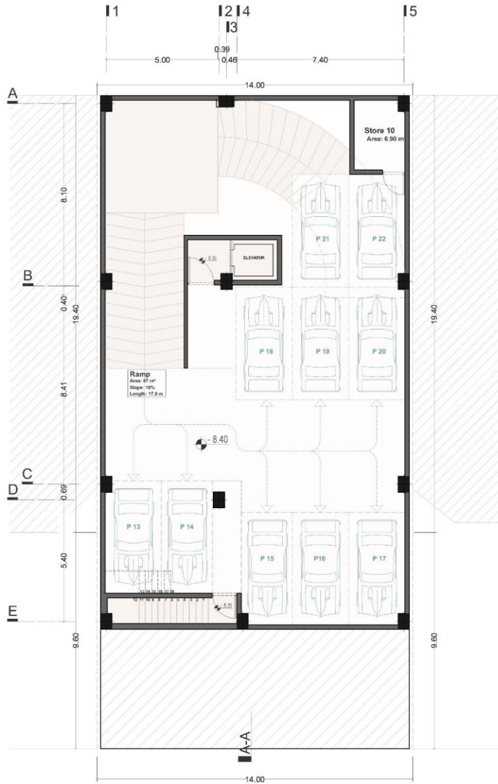
BASEMENT -3 TOTAL AREA: 324.69 m 2 NUMBER OF PARKING: 10
