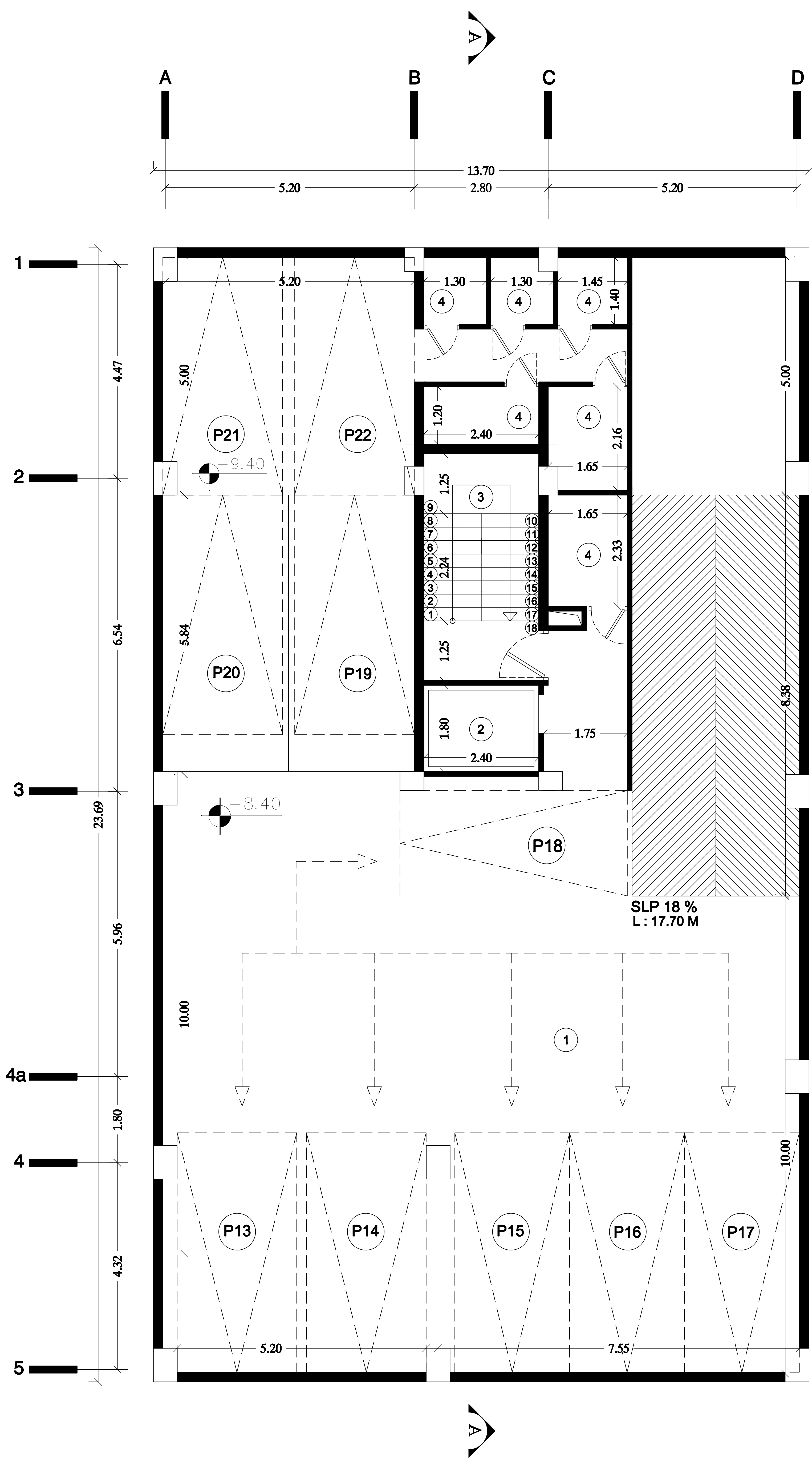
BASMENT FLOOR -3
