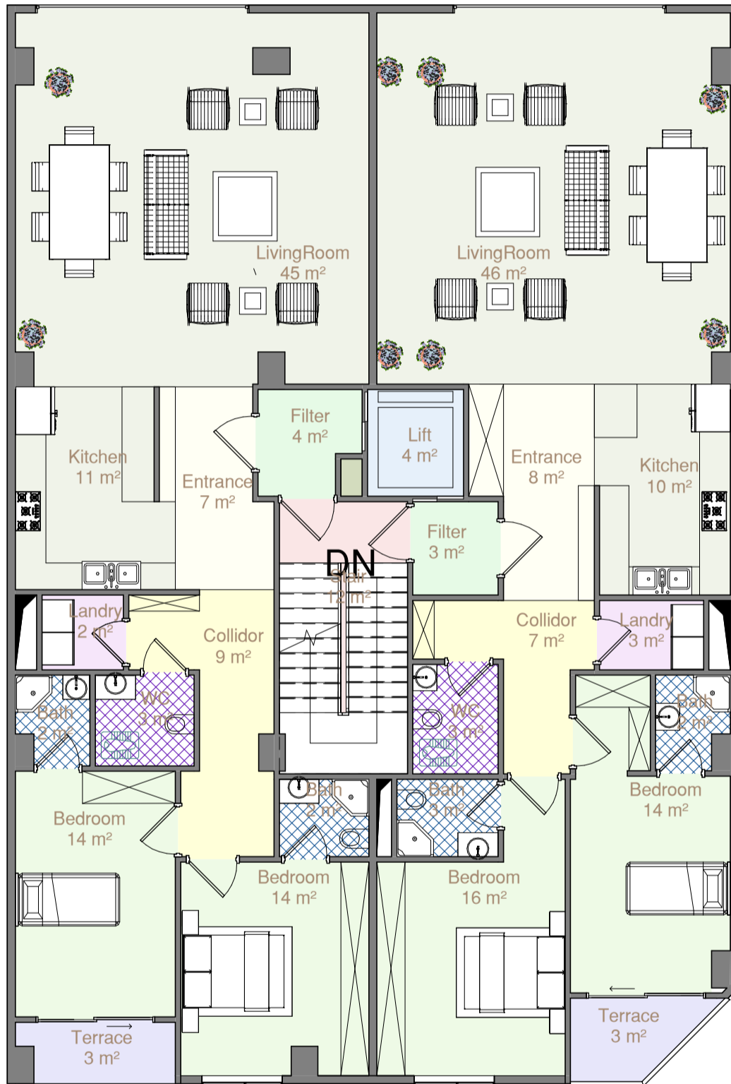
1-5 Furniture Plan Sc: 1/100
