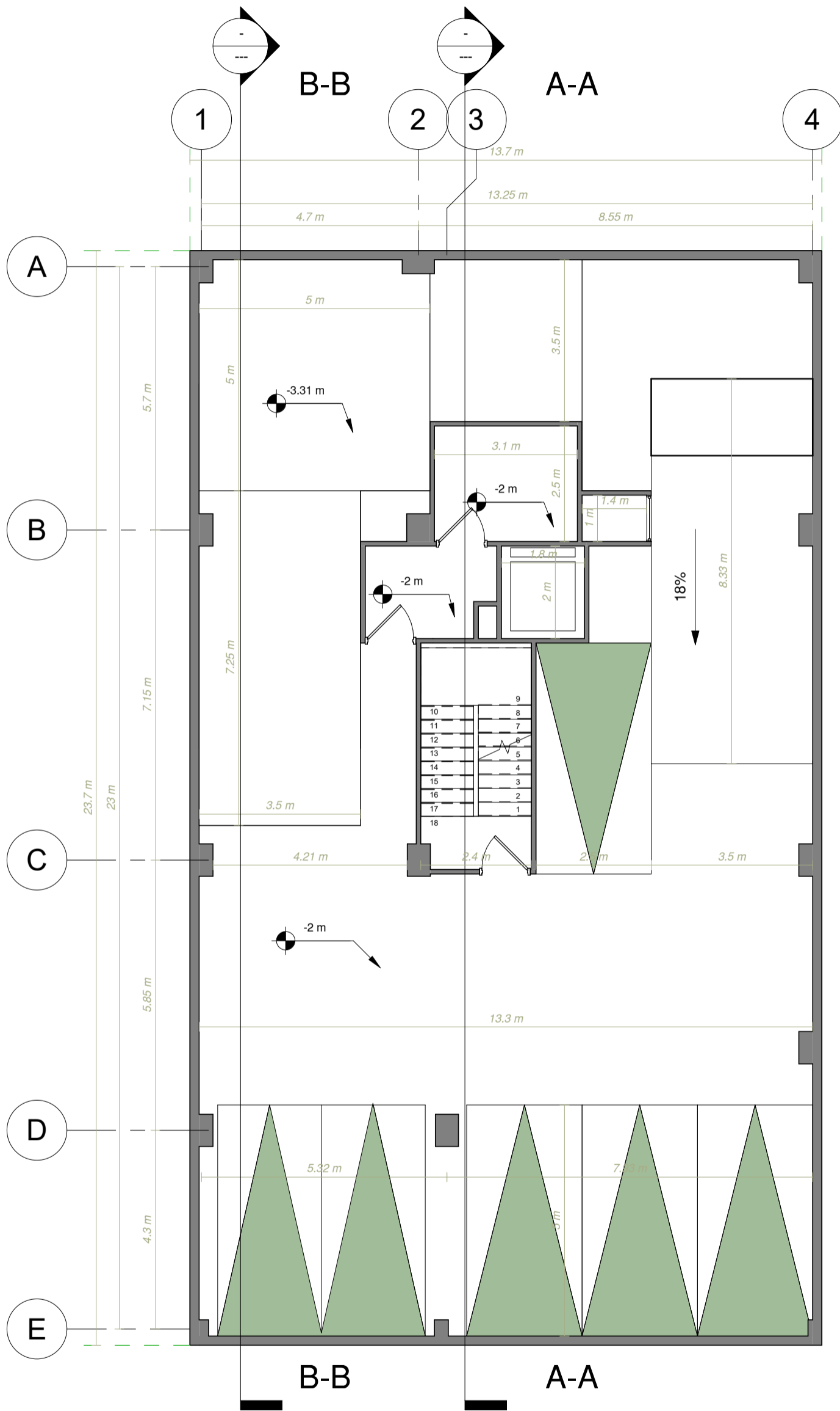
First Basement Dimension Plan Sc: 1/100
