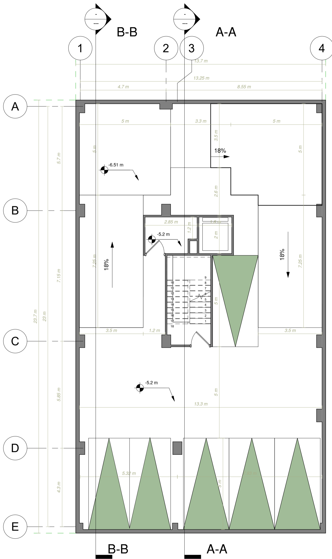
Second Basement Dimension Plan Sc: 1/100
