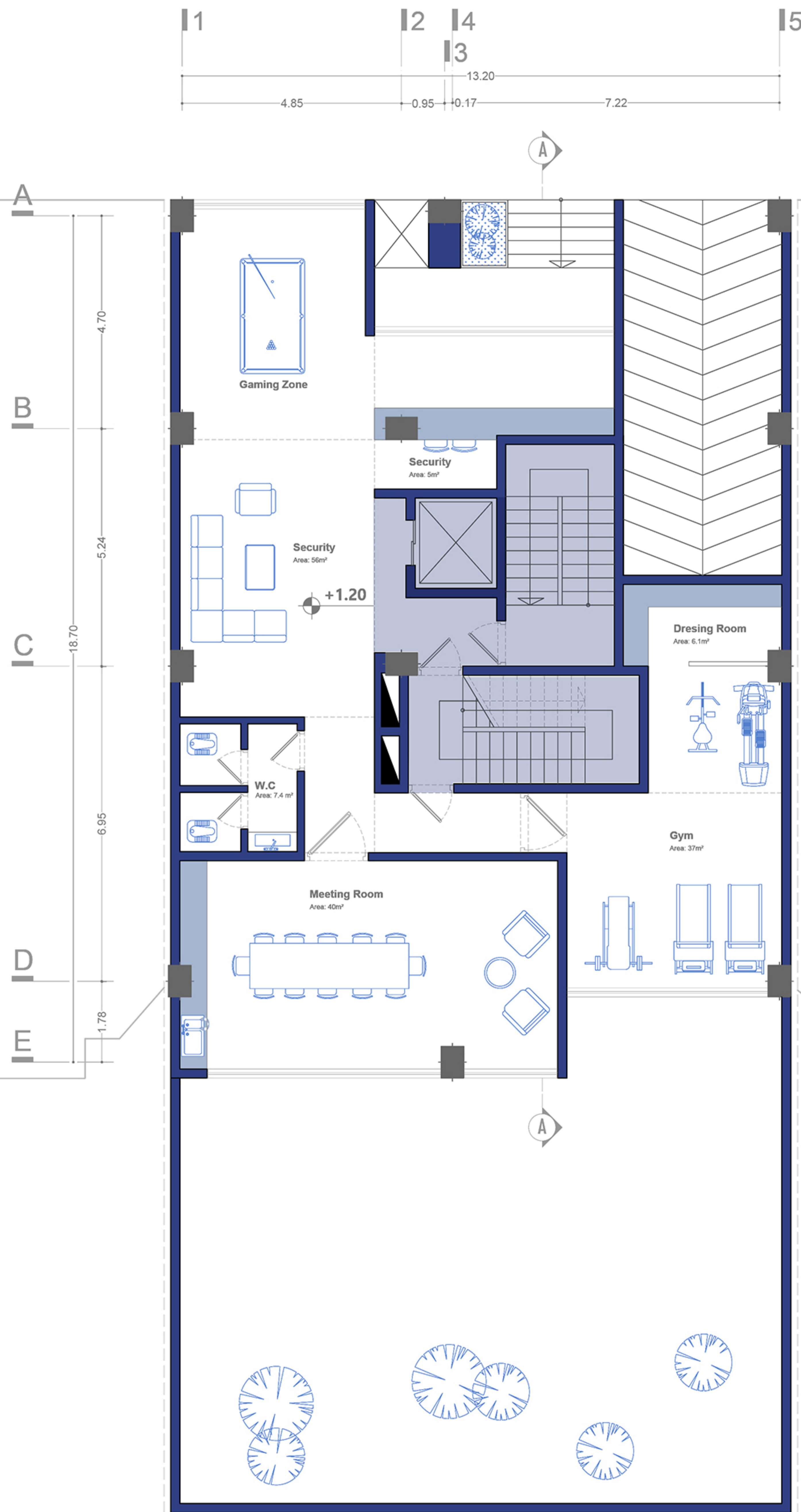
GROUND FLOOR PLAN TOTAL AREA: 220 m²
