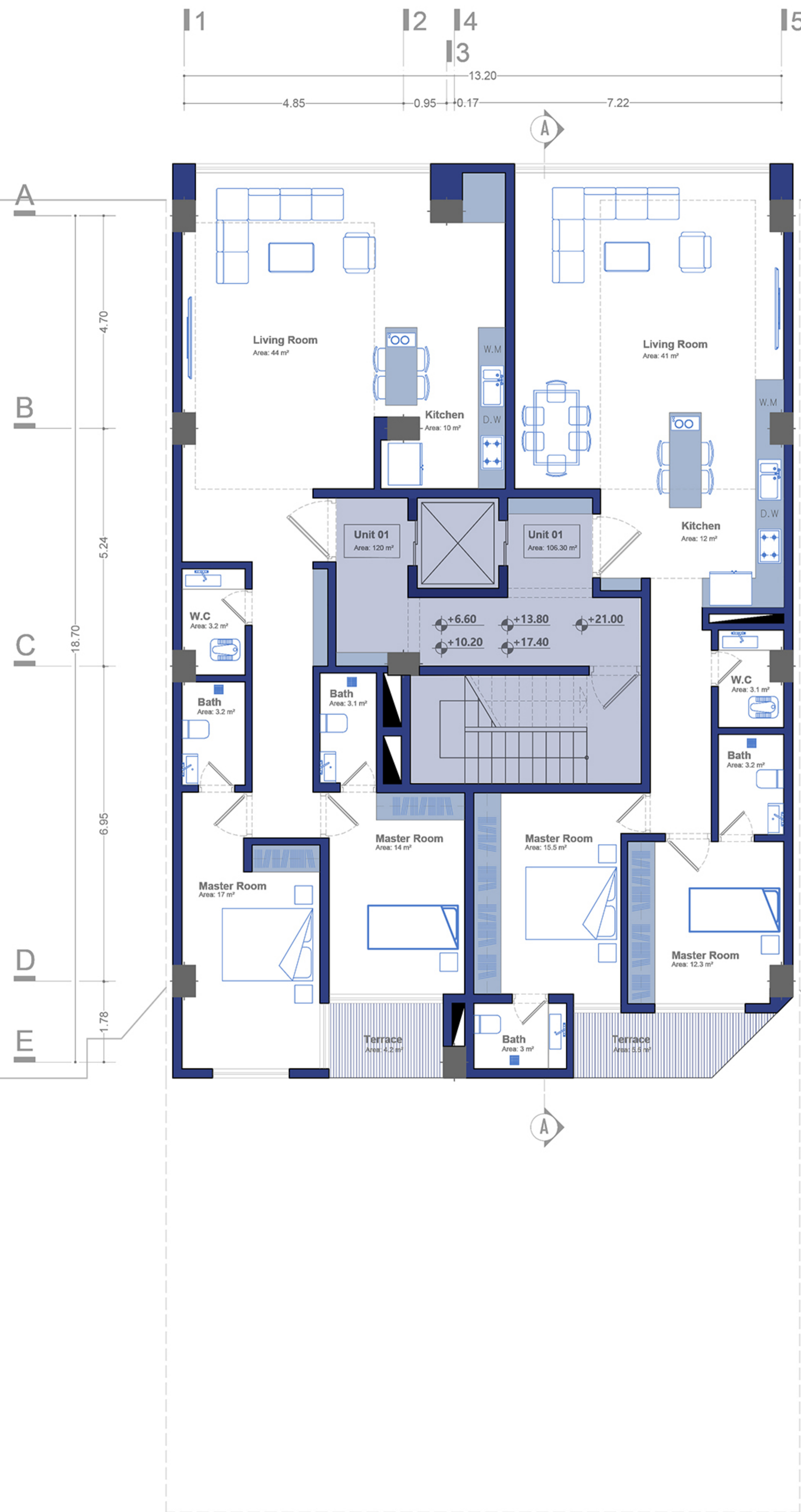
TYPICAL FLOOR PLAN TOTAL AREA: 226.30 m²
