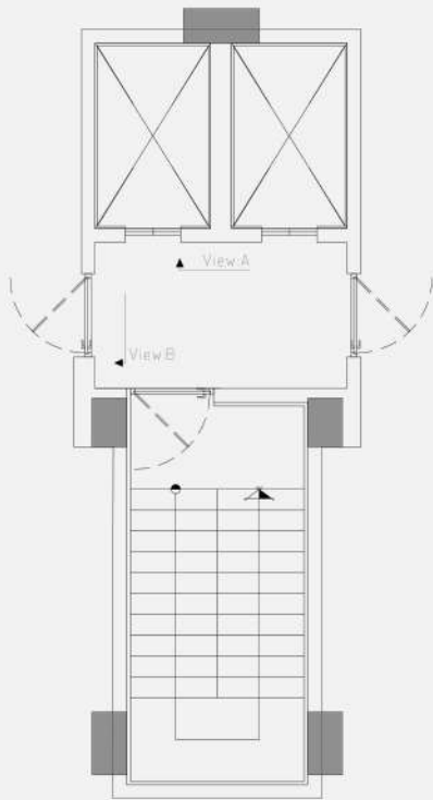
■ Floor Plan
