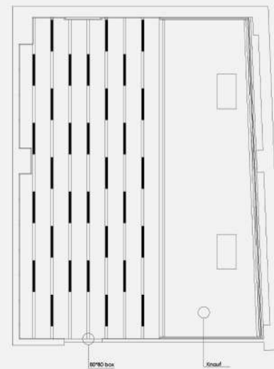
■ Ceiling Plan
